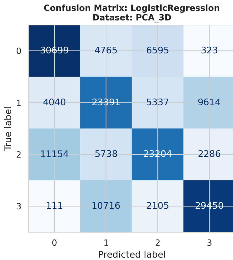
ConfusionMatrix_LogisticRegression_PCA_3D.png
