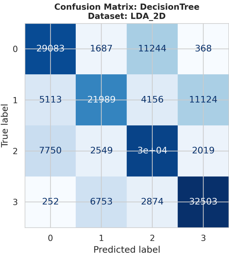
ConfusionMatrix_DecisionTree_LDA_2D.png
