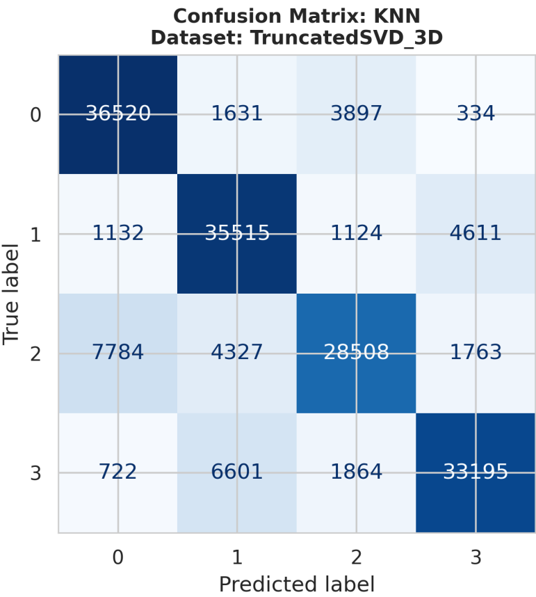
ConfusionMatrix_KNN_TruncatedSVD_3D.png
