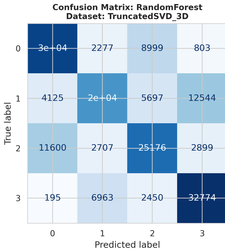
ConfusionMatrix_RandomForest_TruncatedSVD_3D.png
