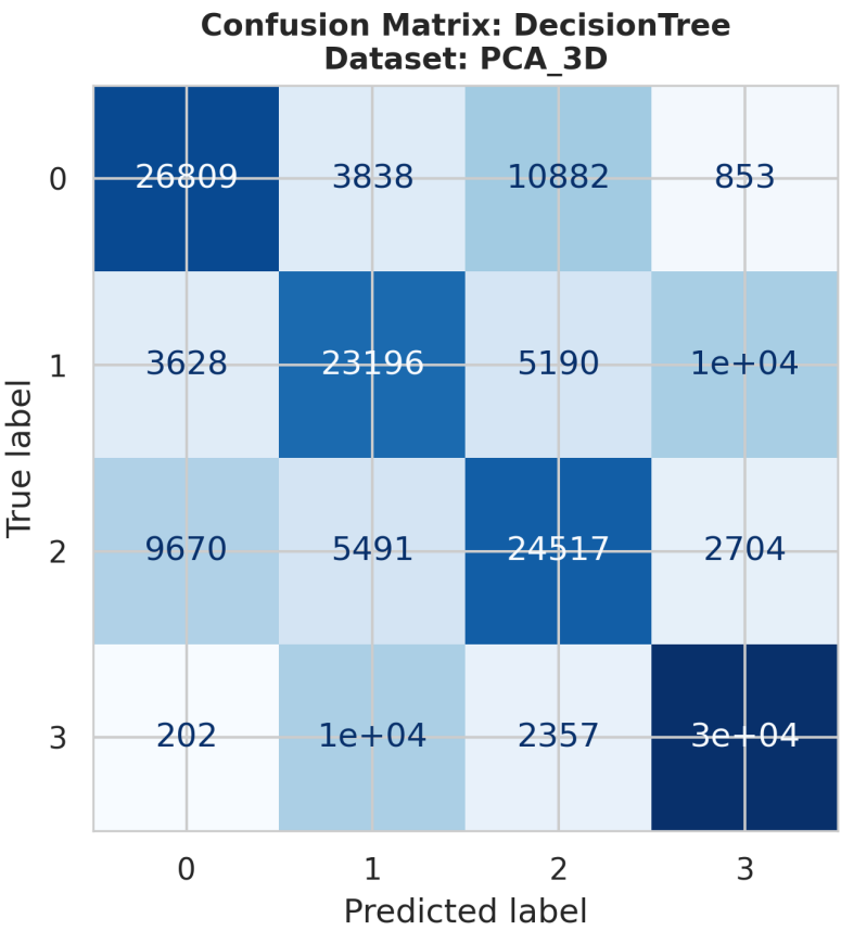
ConfusionMatrix_DecisionTree_PCA_3D.png
