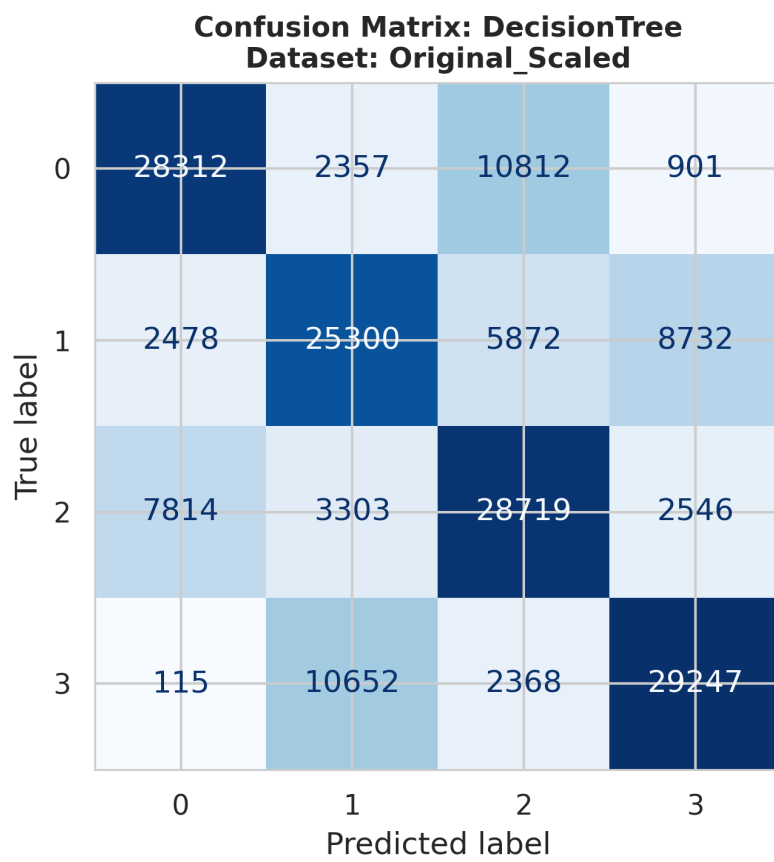
ConfusionMatrix_DecisionTree_Original_Scaled.png
