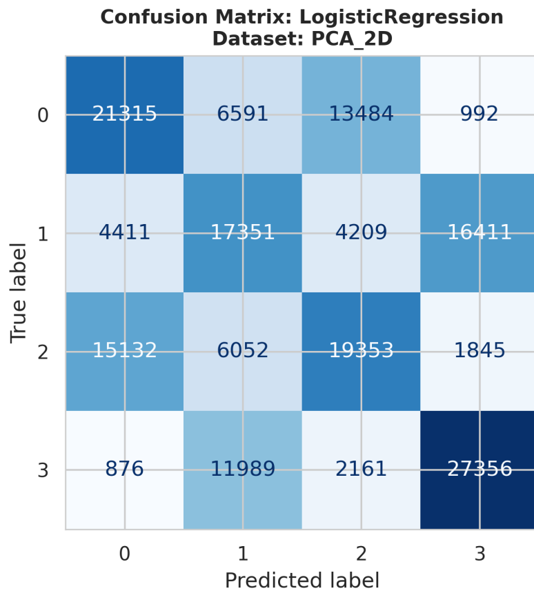
ConfusionMatrix_LogisticRegression_PCA_2D.png
