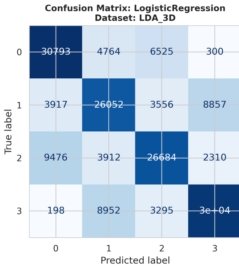
ConfusionMatrix_LogisticRegression_LDA_3D.png
