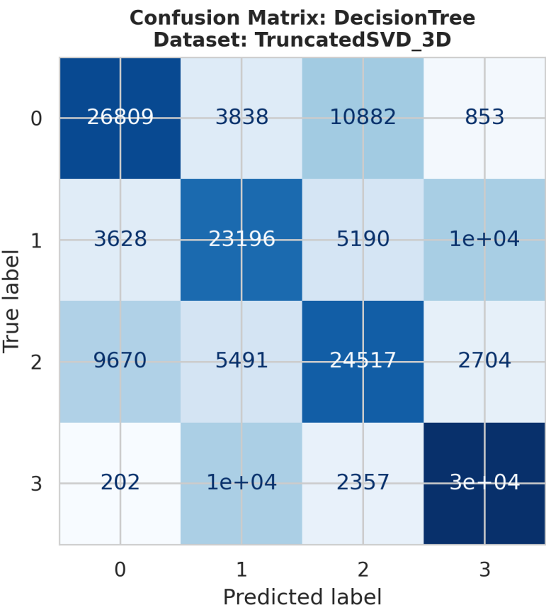
ConfusionMatrix_DecisionTree_TruncatedSVD_3D.png
