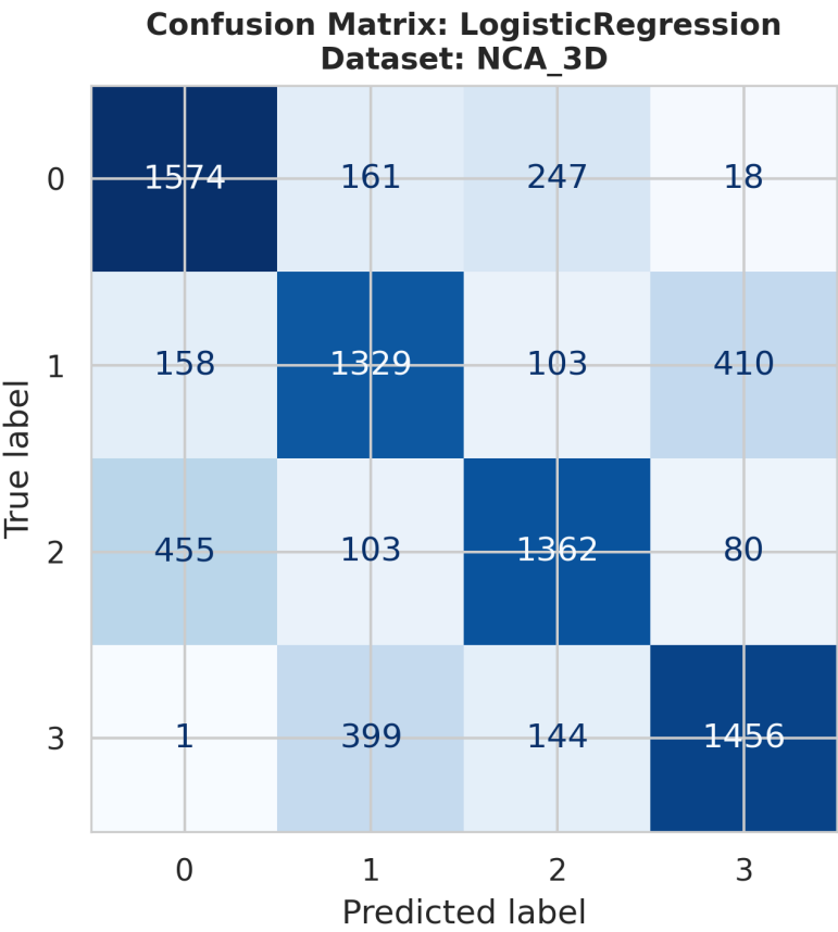
ConfusionMatrix_LogisticRegression_NCA_3D.png
