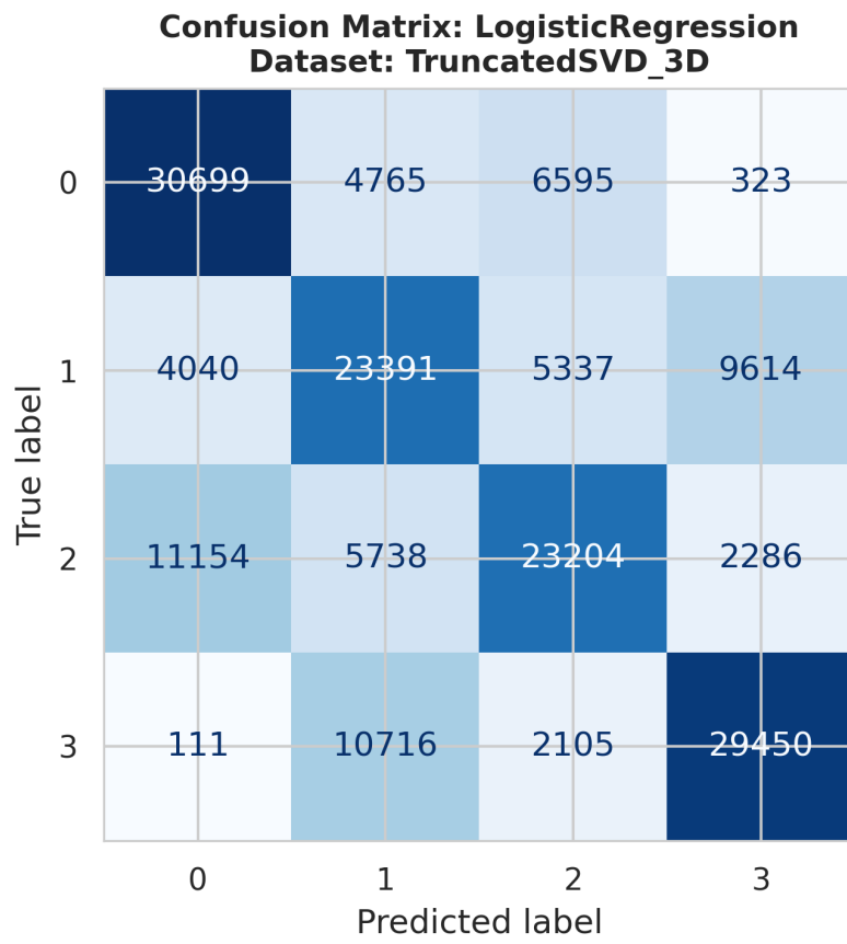
ConfusionMatrix_LogisticRegression_TruncatedSVD_3D.png
