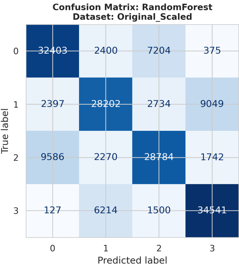
ConfusionMatrix_RandomForest_Original_Scaled.png
