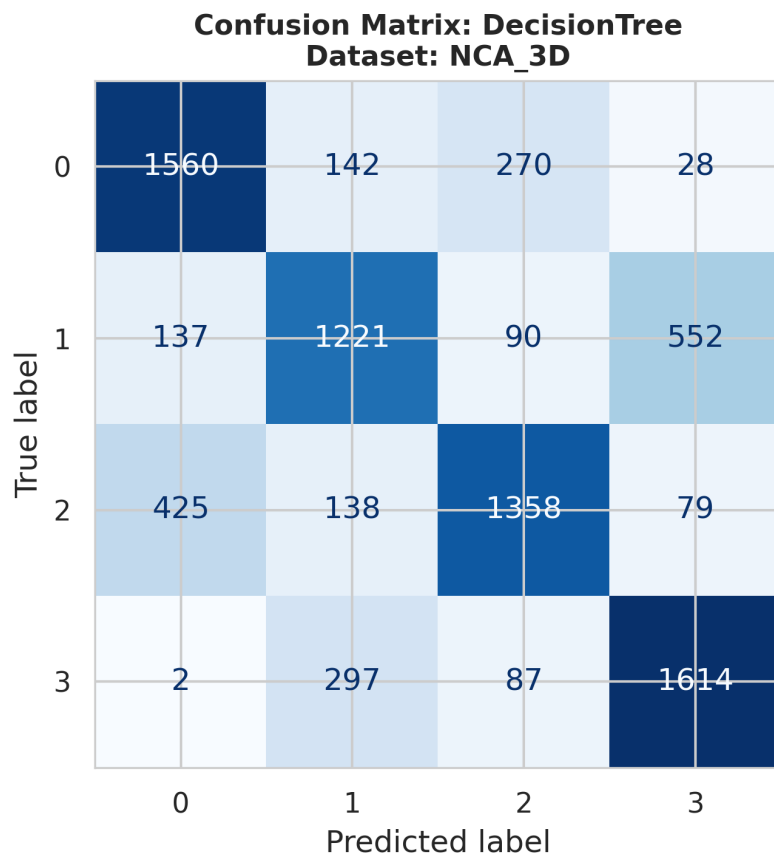
ConfusionMatrix_DecisionTree_NCA_3D.png
