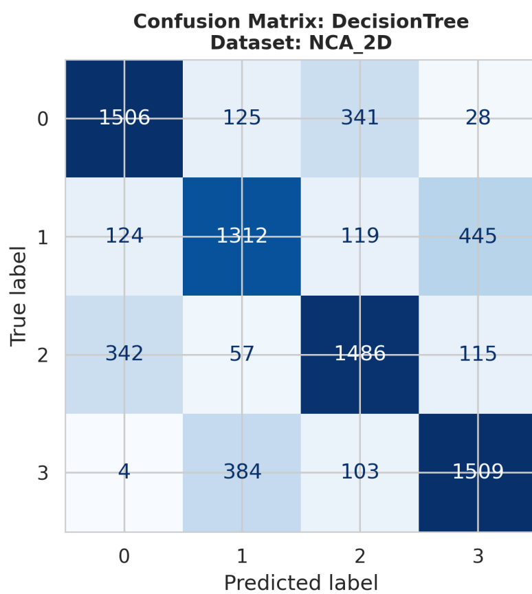
ConfusionMatrix_DecisionTree_NCA_2D.png
