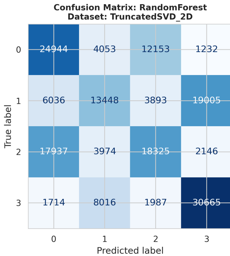
ConfusionMatrix_RandomForest_TruncatedSVD_2D.png
