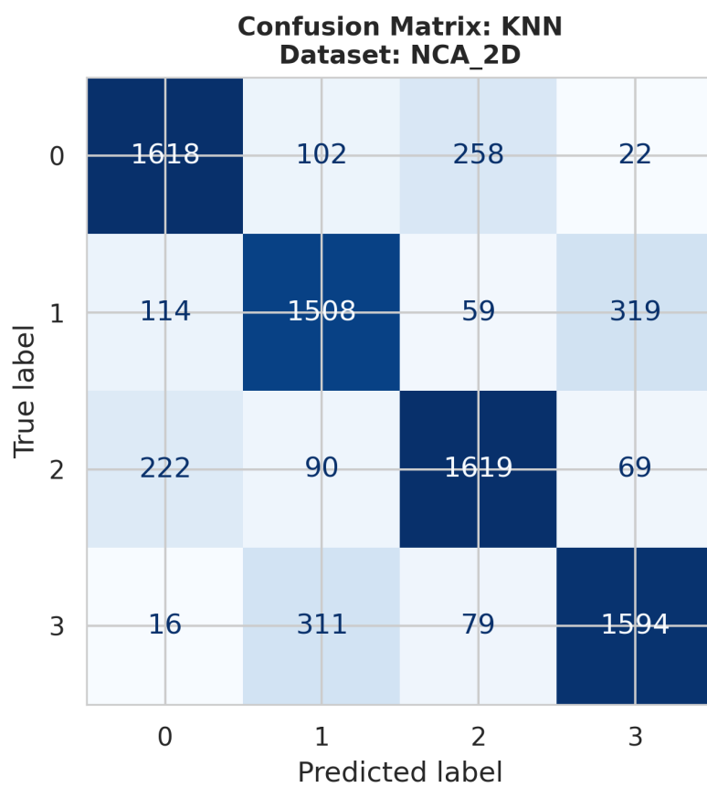
ConfusionMatrix_KNN_NCA_2D.png
