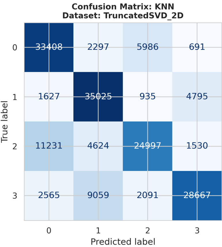
ConfusionMatrix_KNN_TruncatedSVD_2D.png
