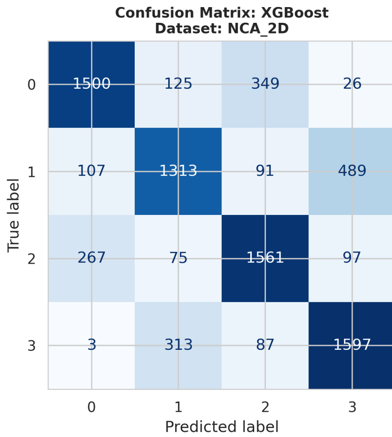
ConfusionMatrix_XGBoost_NCA_2D.png
