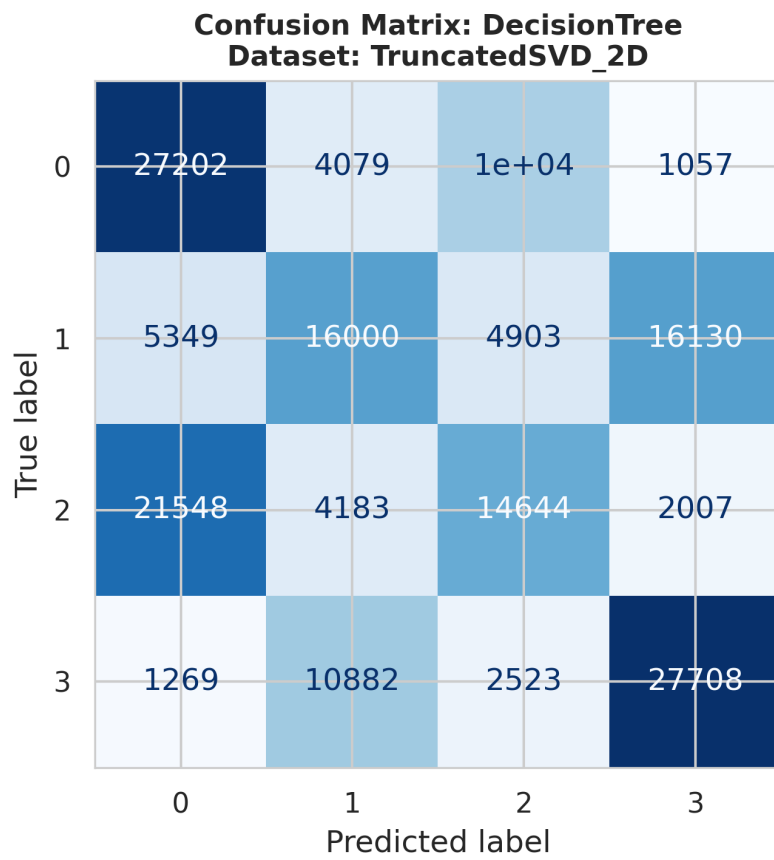
ConfusionMatrix_DecisionTree_TruncatedSVD_2D.png
