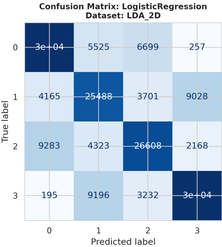
ConfusionMatrix_LogisticRegression_LDA_2D.png
