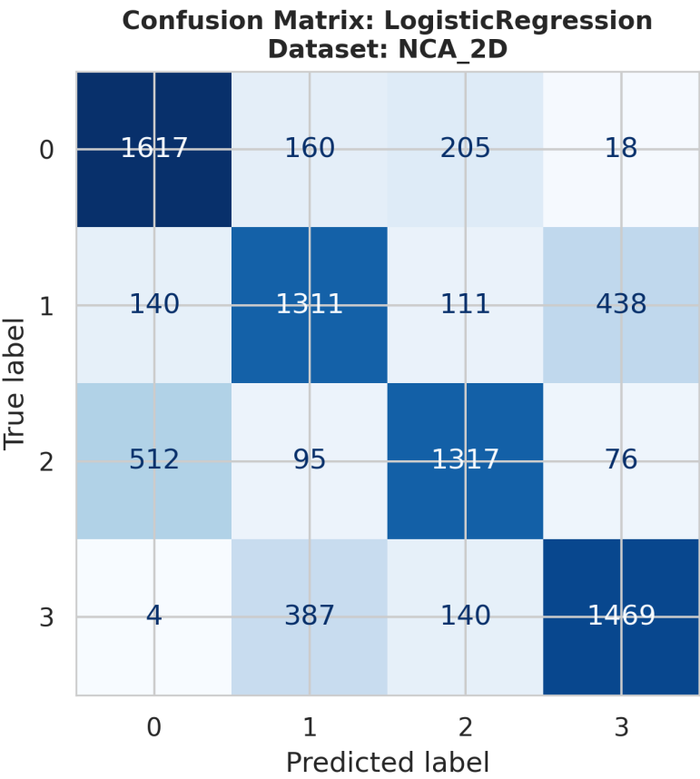
ConfusionMatrix_LogisticRegression_NCA_2D.png
