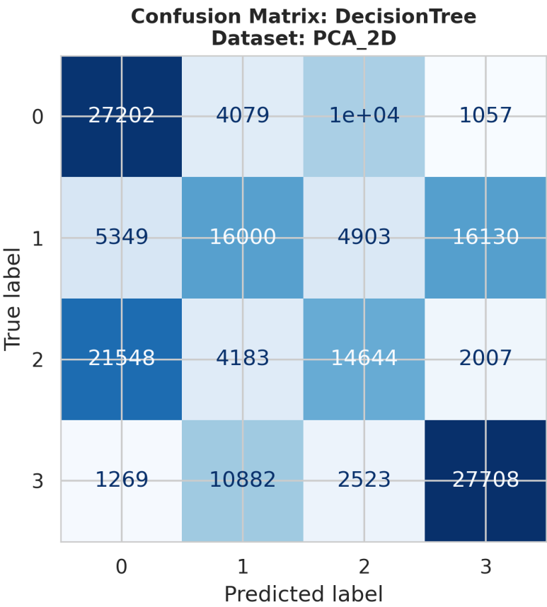
ConfusionMatrix_DecisionTree_PCA_2D.png
