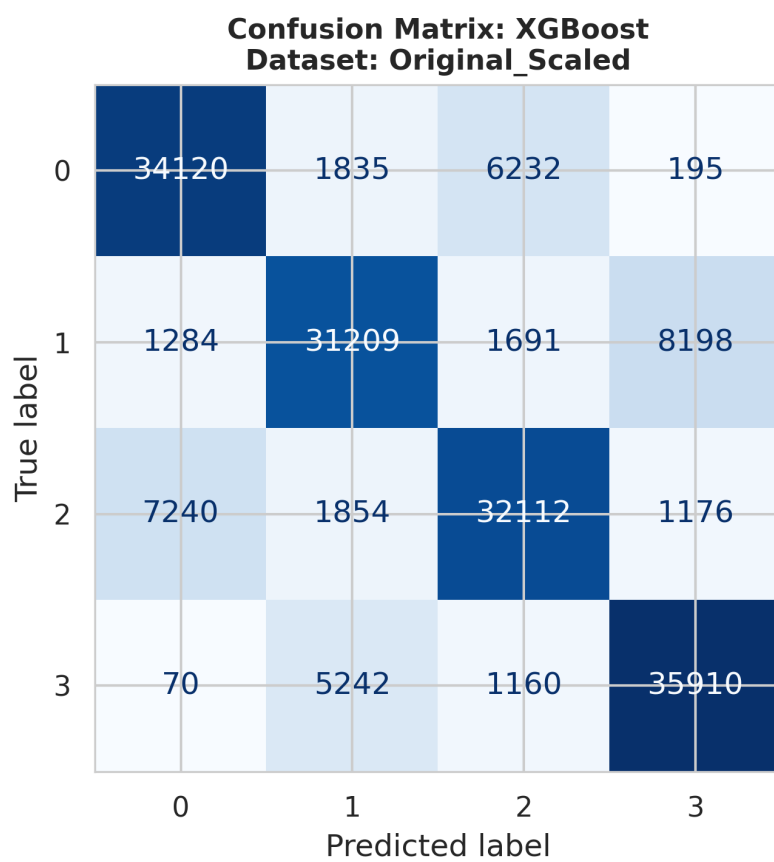
ConfusionMatrix_XGBoost_Original_Scaled.png
