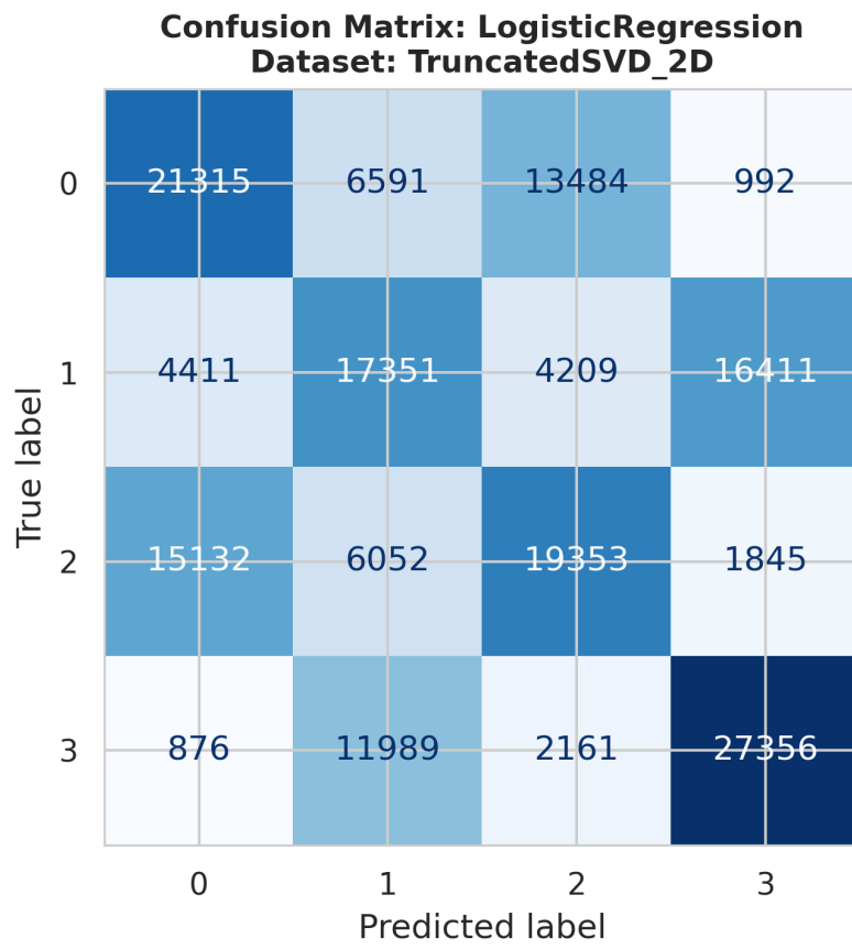
ConfusionMatrix_LogisticRegression_TruncatedSVD_2D.png
