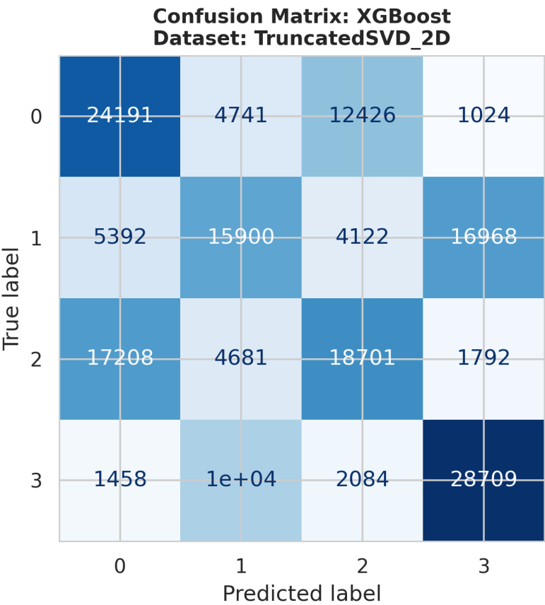
ConfusionMatrix_XGBoost_TruncatedSVD_2D.png
